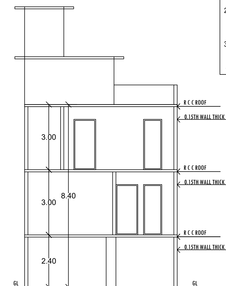
SECTION X-X
